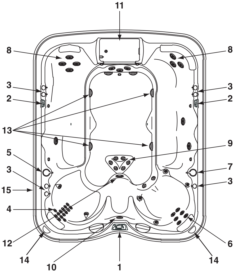
Figure -F Hot Tub Top View
