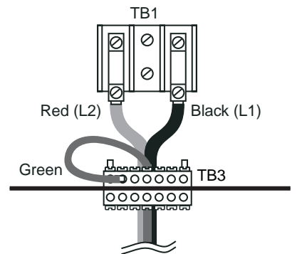
Figure-C Terminal Block 240V Wire Connection
